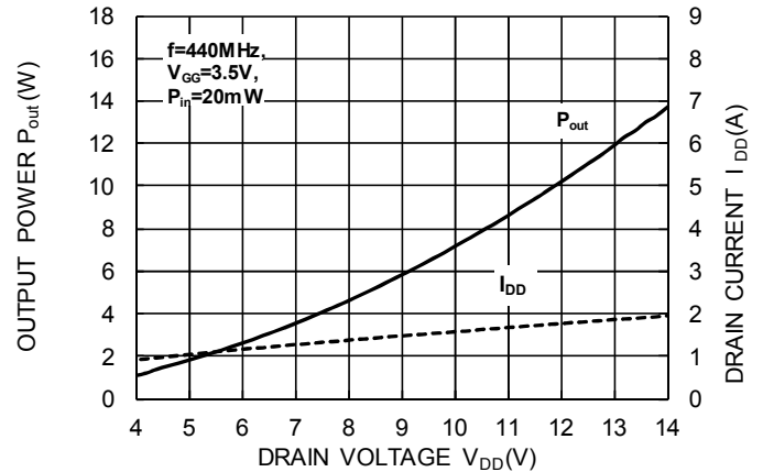
OUTPUT POWER, and DRAIN versus DRAIN VOLTAGE
