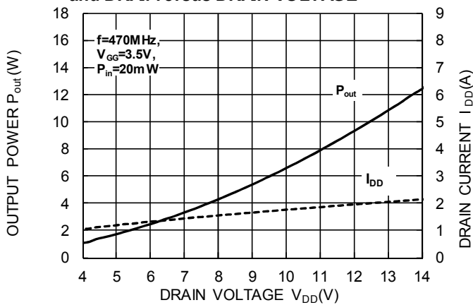
OUTPUT POWER, and DRAIN versus DRAIN VOLTAGE
