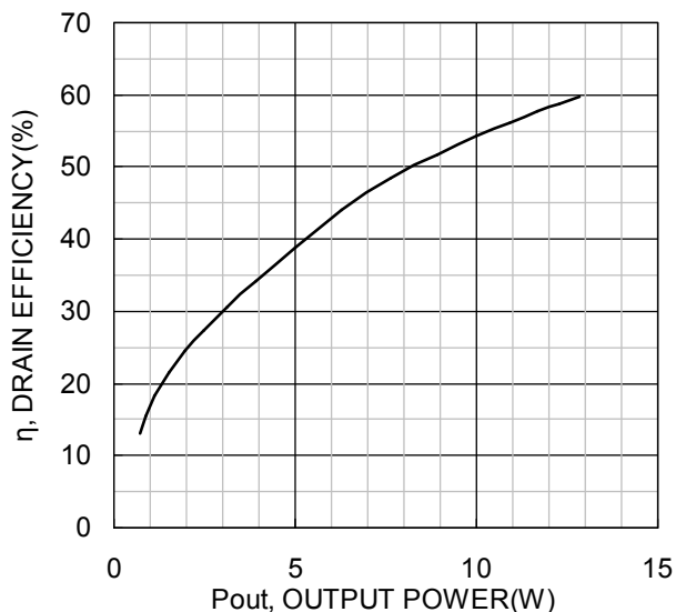
Ta=+25deg.C, Vds=7.2V, Idq=0.30A
