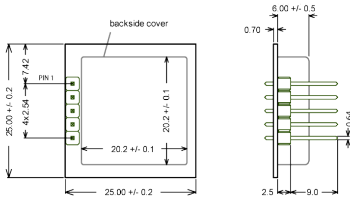
Fig. 3: Mechanical data
